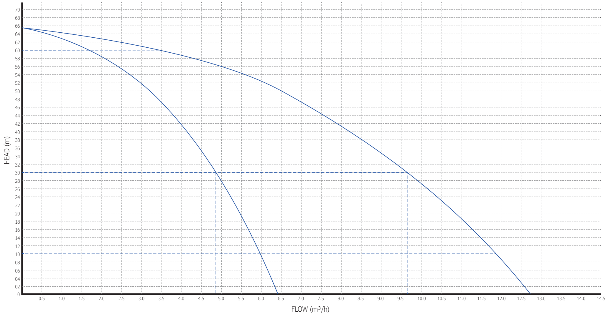
Arlington AiS unit pump performance curves. Single and twin units
